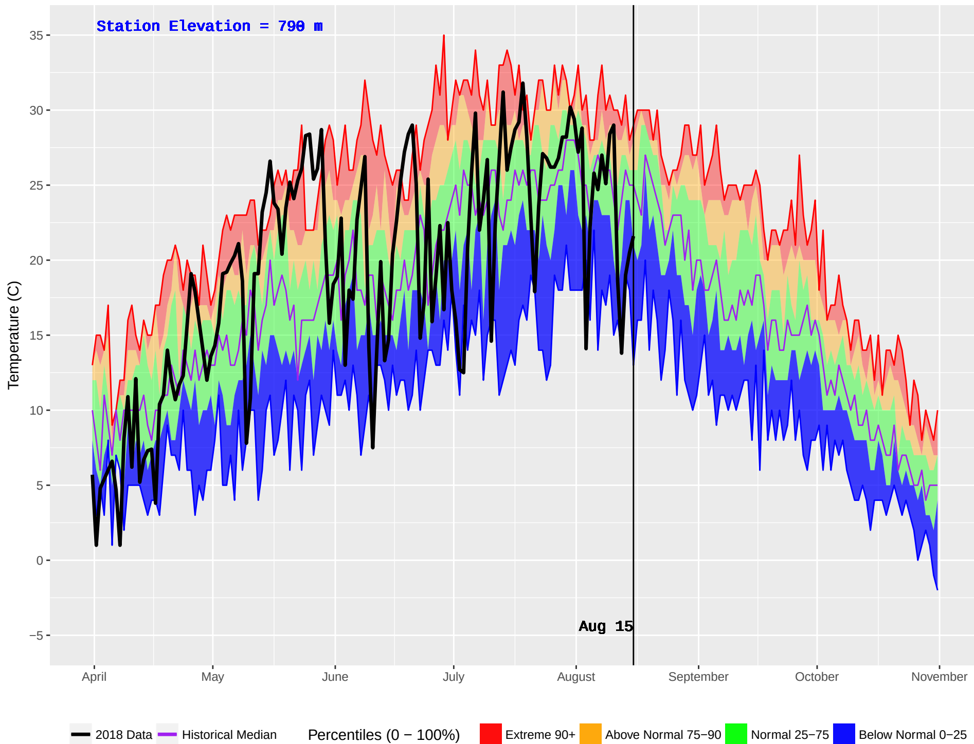
FALLS CREEK (383) : Historical (2002–2016) and Current (2018) Daily Temperature
