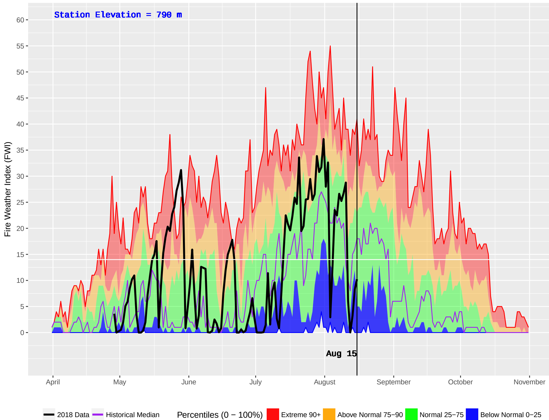
FALLS CREEK (383) : Historical (2002–2016) and Current (2018) Daily Fire Weather Index (FWI)
